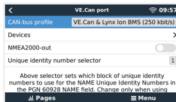
GX screen showing the CAN-bus profile setting
